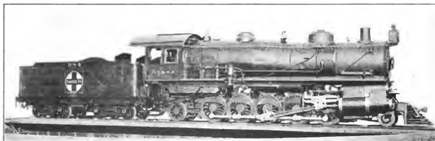
Fig. 48. Ten-Coupled and Trailing Truck (2-10-2) Tandem Compound Locomotive. Built by the Baldwin Locomotive Works for the Atchison, Topeka & Santa Fe. Cylinders 19 in. and 32 in. x 32 in., Working Steam Pressure 225 lbs. per sq. in., Total Heating Surface 4,796 sq. ft., Diameter of Drivers 57 in., Weight on Drivers 234,580 lbs., Total Weight 287,240 lbs.
